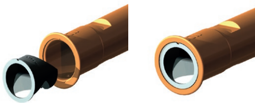
The CONVECTROL is simply inserted torsion safe into a combination fitting
