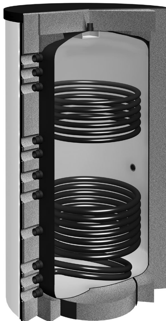
Abb. 1 RATIO Pufferspeicher
