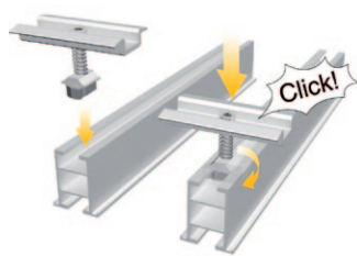
Modulklemme TRIC clip
